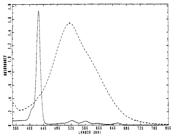
Figure 1. Visible spectra of 1-P (continuous line) and 2-P (broken line), the latter multiplied by 4.0, at equal concentrations ( 3.5 \times 10^{-6} mol \text{dm}^{-3} ) in chloroform solution. The solution of 2-P was obtained by oxidation of a stock solution of 1-P ( 5 \times 10^{-6} mol) in chloroform ( 5 \text{ cm}^3 ) using a solution of m -chloroperbenzoic acid ( 5 \times 10^{-6} mol) in chloroform and chelated protohemin (0.3 mg) catalyst.
