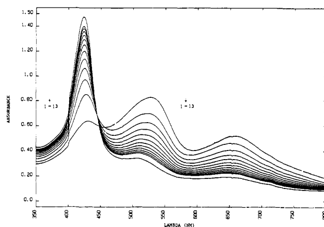
Figure 3. Spectral changes accompanying the reduction of 2-Fe by p -cresol ( 2.0 \times 10^{-3} mol \text{dm}^{-3} ) in benzene solution containing 1-methylimidazole (0.2 mol \text{dm}^{-3} ) at 30 °C. Time intervals between scans 1–12 are 2 min each and the final spectrum, 13, was recorded after 3 h.
