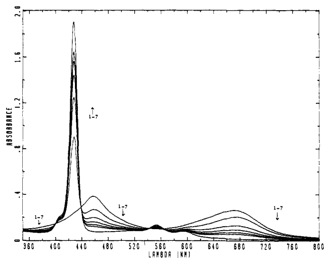
Figure 2. Spectral changes accompanying the reduction of 2-Zn to 1-Zn by p -cresol ( 7.9 \times 10^{-4} mol \text{dm}^{-3} ) in chloroform solution at 30 °C. Time intervals between scans 1–6 are 6.5 min each and the final spectrum, 7, was recorded after 3 h.
